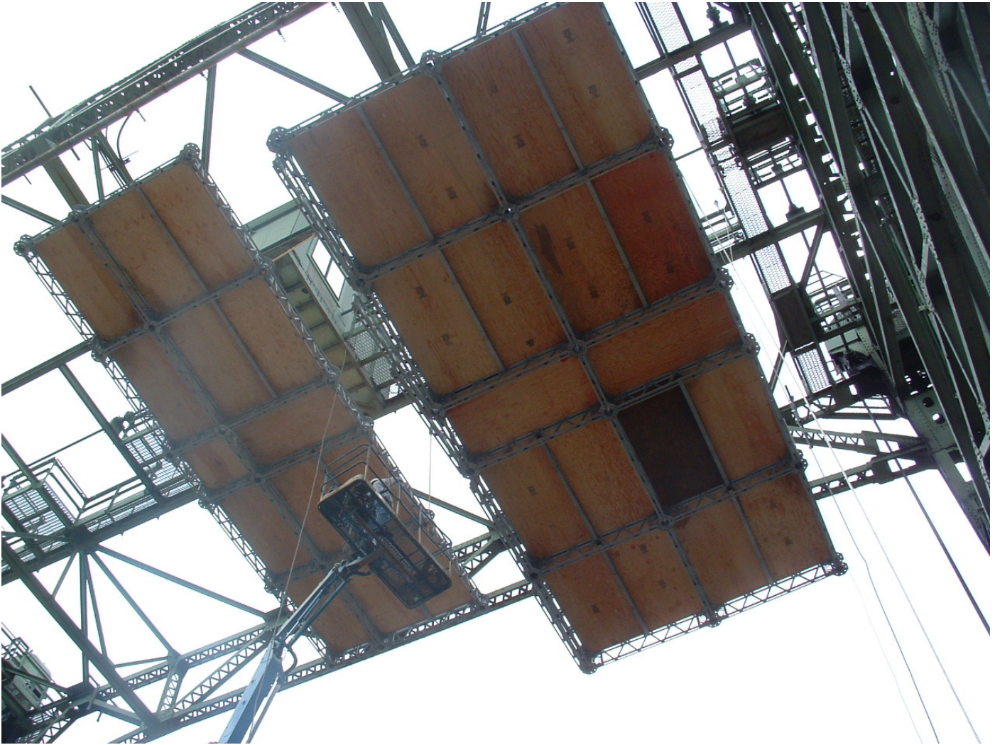
Rte 44 Lift Span Bridge Over Mantua Creek 2 nd Partial Quik Deck Platform Being Lifted Into Place Upper Level
